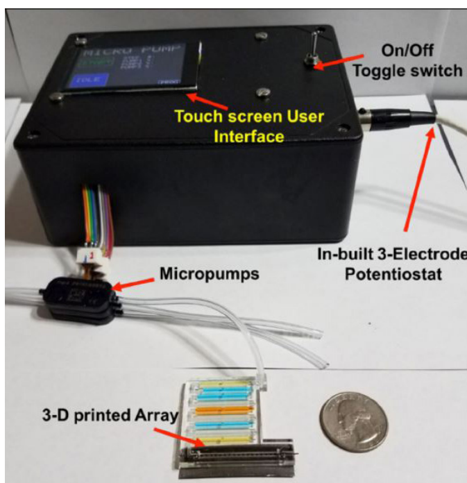
A prototype automated blood test with low-cost 3D-printed array for cancer detection (image courtesy of Dr. James Rusling; quarter for scale)
